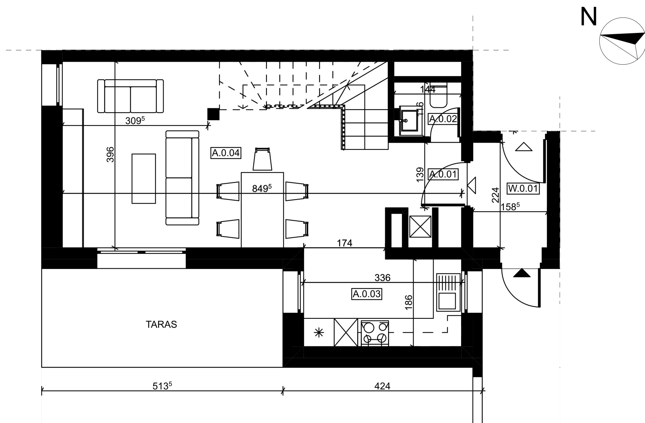
0. Parter 1:50
