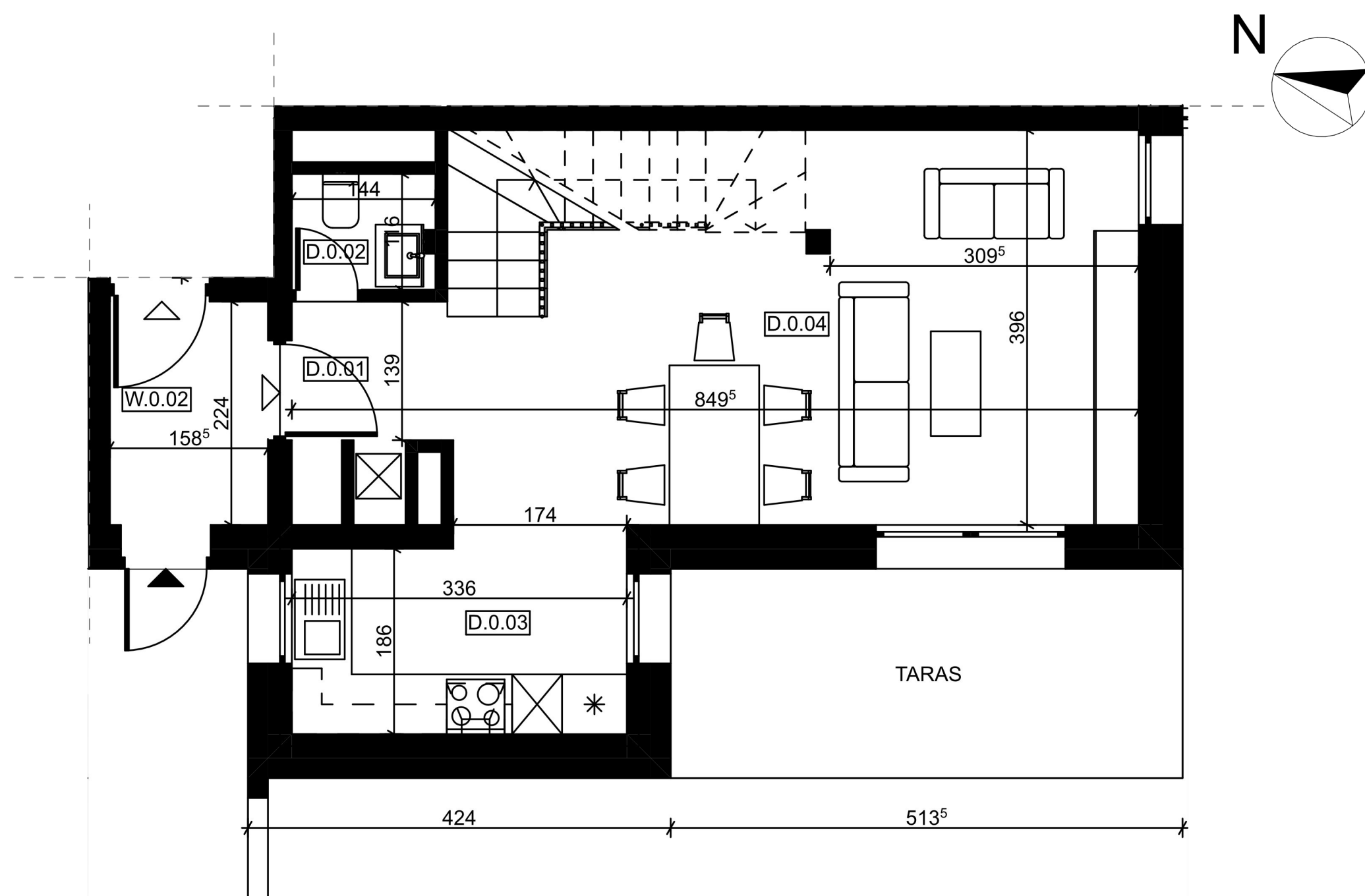
0. Parter 1:50
